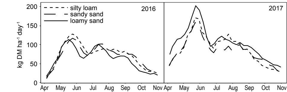
Figure 2. Daily pasture growth rates (kg DM ha -1 day -1 ) of the examined sites in 2016 and 2017 with N-fertilisation of 280 kg N ha -1 y -1 .
