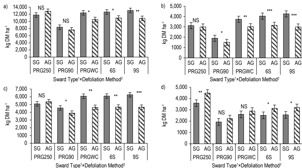
Figure 1. The effect of sward type and defoliation method on the (a) annual (b) spring (c) summer (d) autumn DM production (kg DM ha -1 ; least square means \pm SEM as error bars).
